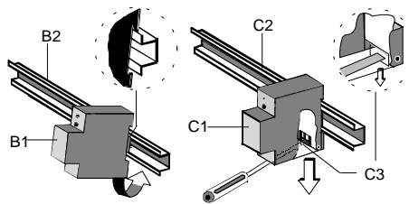
Figure 2: Mounting and dismounting a DIN-rail device
