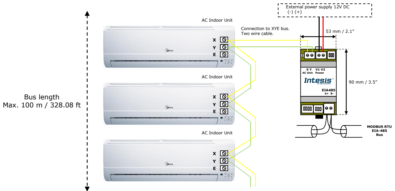
Figure 2.2 INMBSMID004I000 / INMBSMID008I000 / INMBSMID032I000 connection diagram
